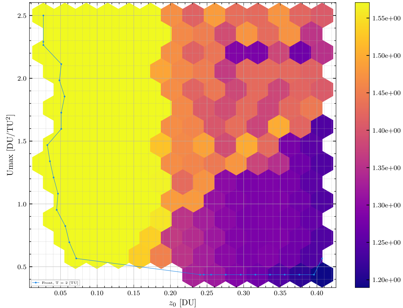
Cone angles [rad] over constant period, T = 2 [TU]
